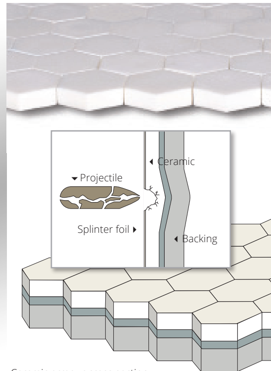
Ceramic armour cross section
